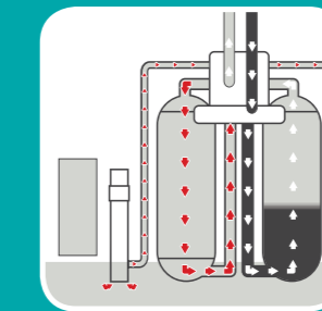
While tank A regenerates, tank B continues to produce soft water.
