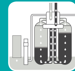
After regeneration (10 mins) tank A returns to continue softening water.
