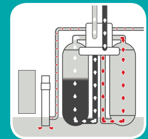
When tank B regenerates, tank A continues to produce soft water.
