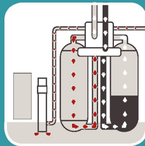
While tank A regenerates, tank B continues to produce soft water
